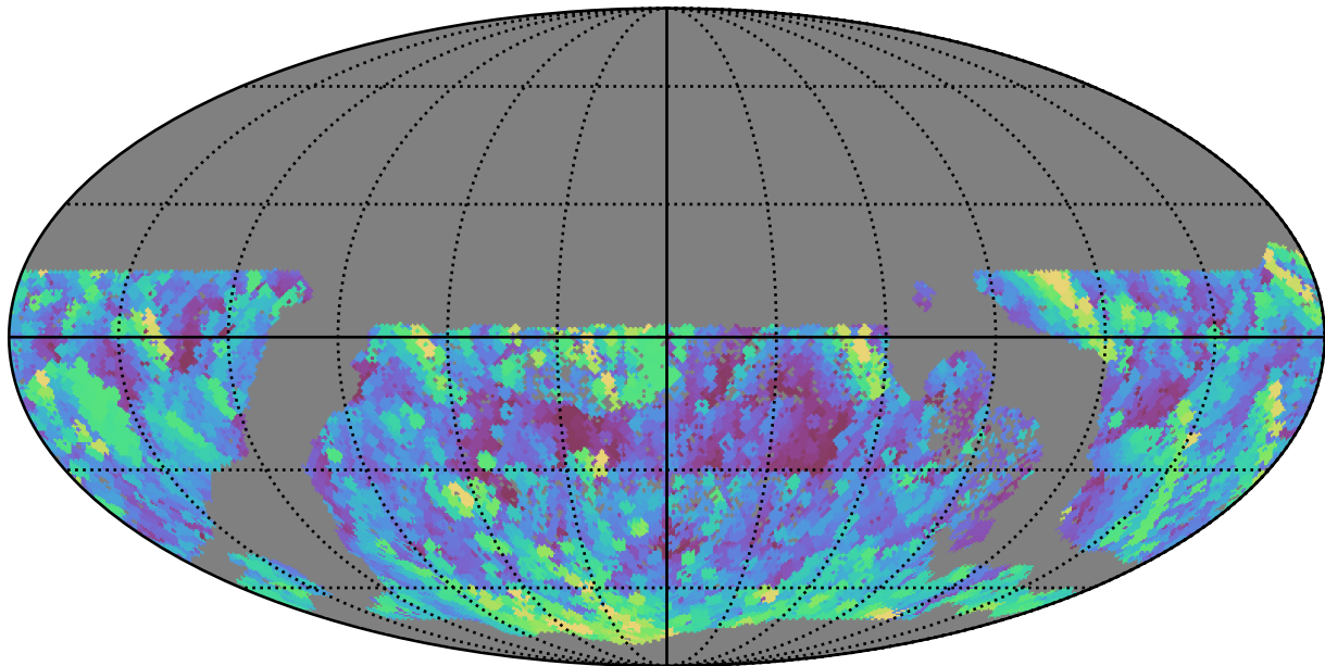
too_combined_s0.5_v3.4_10yrs WFD g band: Max airmass
