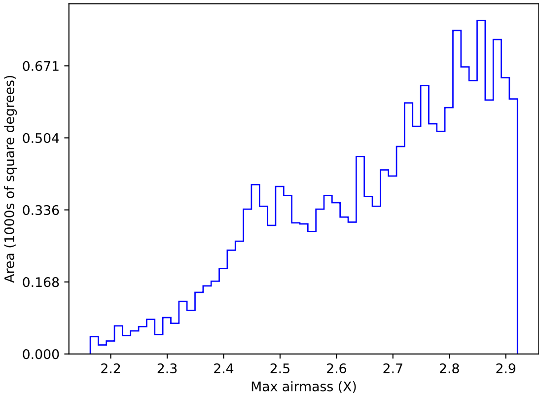
too_combined_s0.5_v3.4_10yrs WFD all bands: Max airmass
