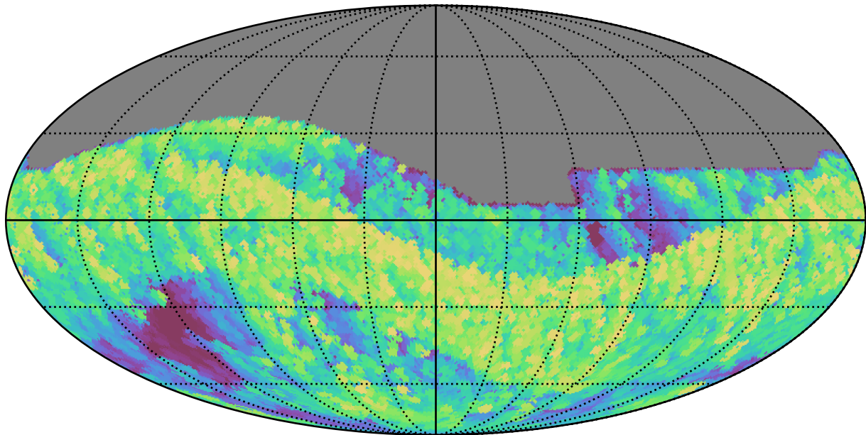
too_combined_s0.5_v3.4_10yrs All sky z band: Max airmass
