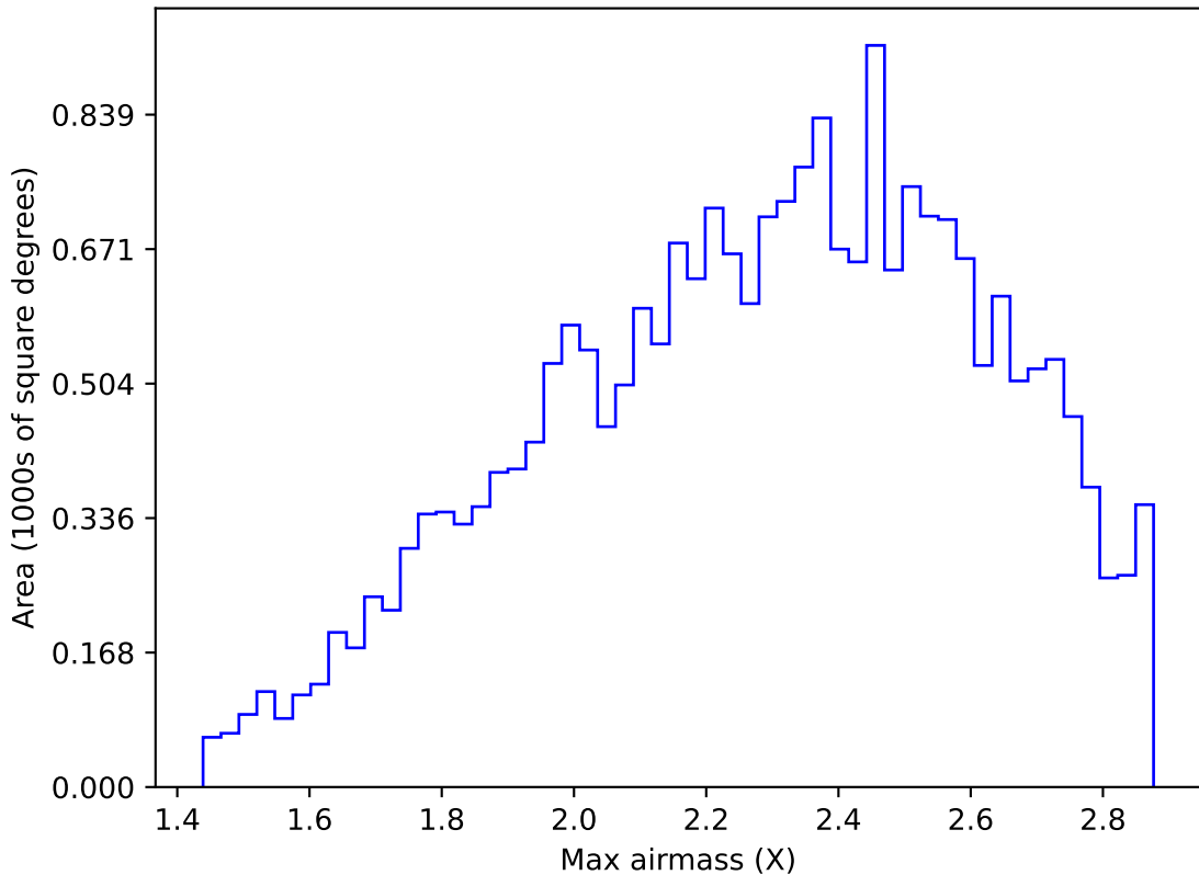
too_combined_s0.5_v3.4_10yrs All sky y band: Max airmass
