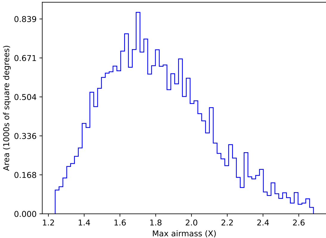
too_combined_s0.5_v3.4_10yrs All sky u band: Max airmass
