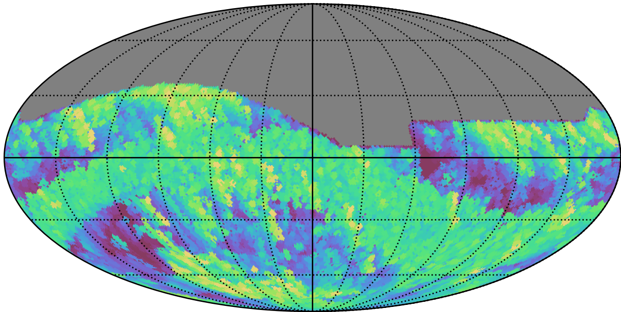
too_combined_s0.5_v3.4_10yrs All sky r band: Max airmass
