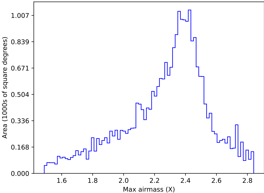
too_combined_s0.5_v3.4_10yrs All sky r band: Max airmass
