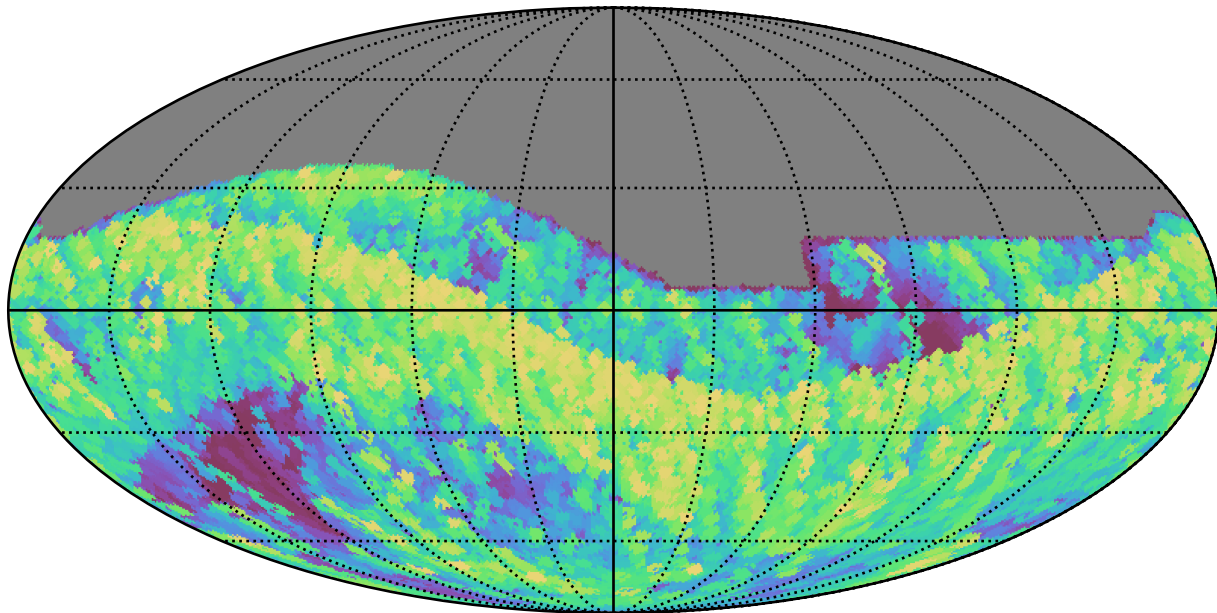
too_combined_s0.5_v3.4_10yrs All sky i band: Max airmass
