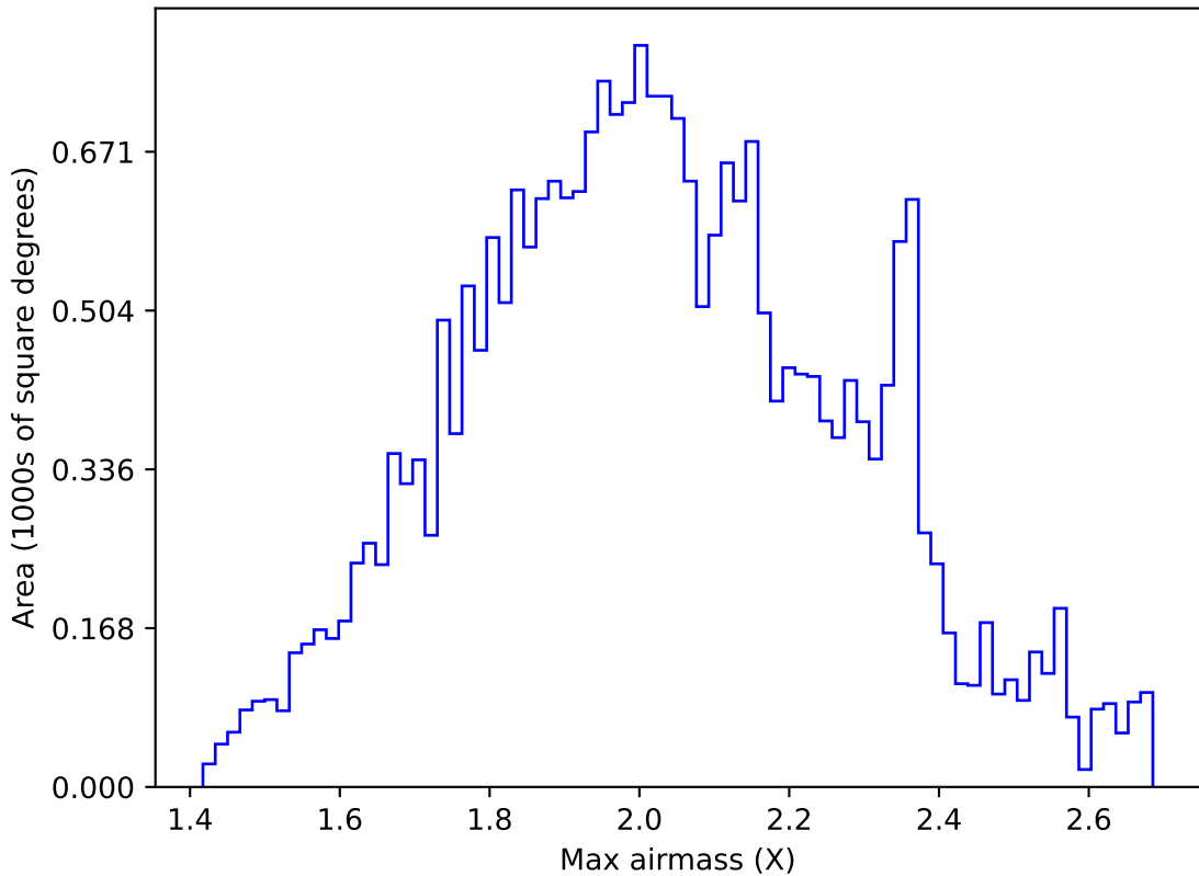
too_combined_s0.5_v3.4_10yrs All sky g band: Max airmass
