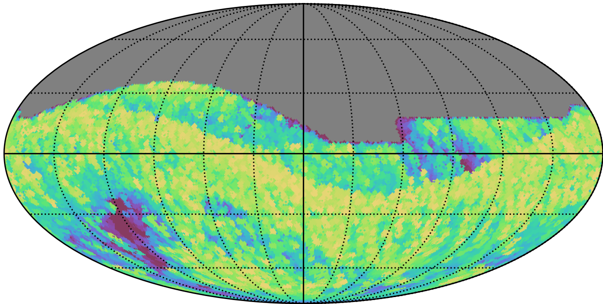
too_combined_s0.5_v3.4_10yrs All sky all bands: Max airmass
