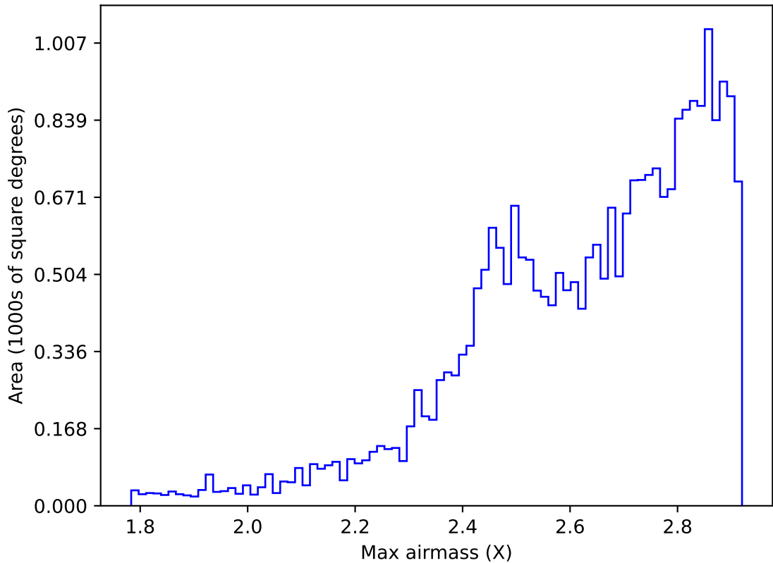
too_combined_s0.5_v3.4_10yrs All sky all bands: Max airmass
