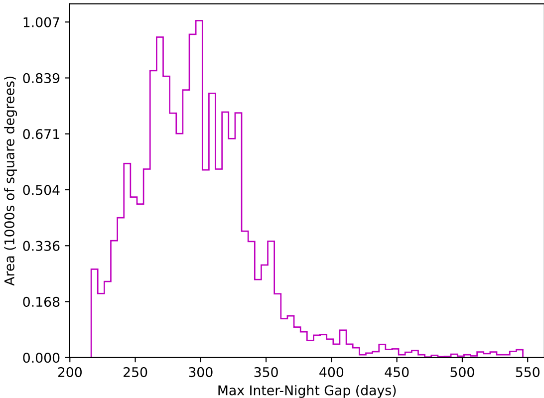
too_combined_s0.5_v3.4_10yrs WFD z band: Max Inter-Night Gap
