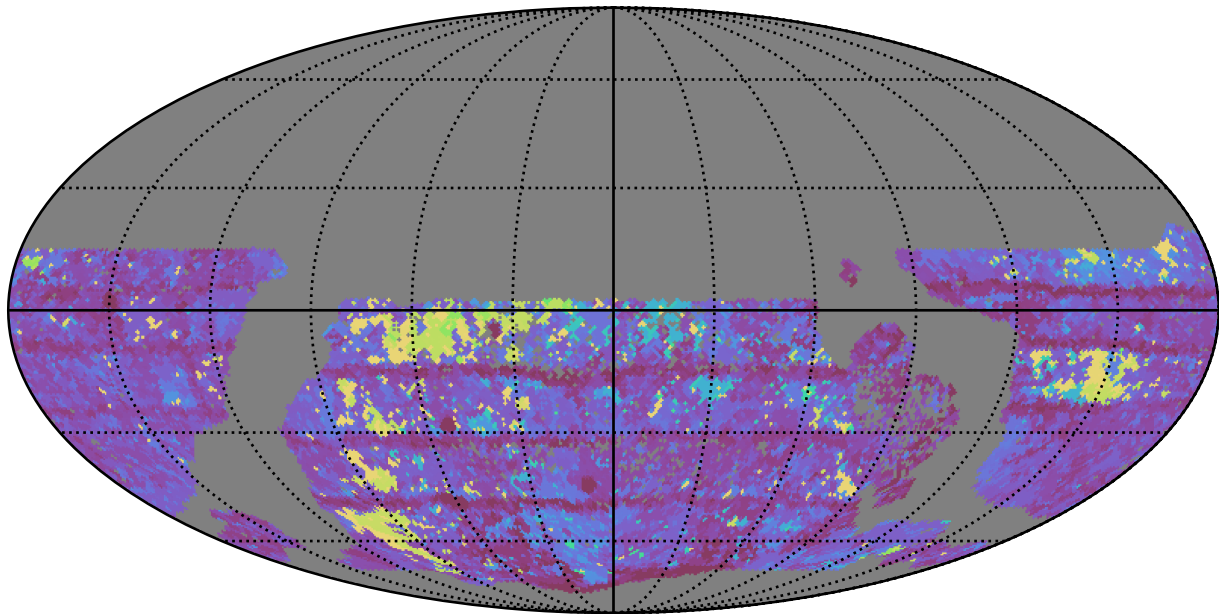
too_combined_s0.5_v3.4_10yrs WFD y band: Max Inter-Night Gap
