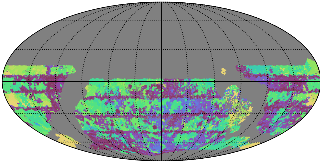
too_combined_s0.5_v3.4_10yrs WFD u band: Max Inter-Night Gap
