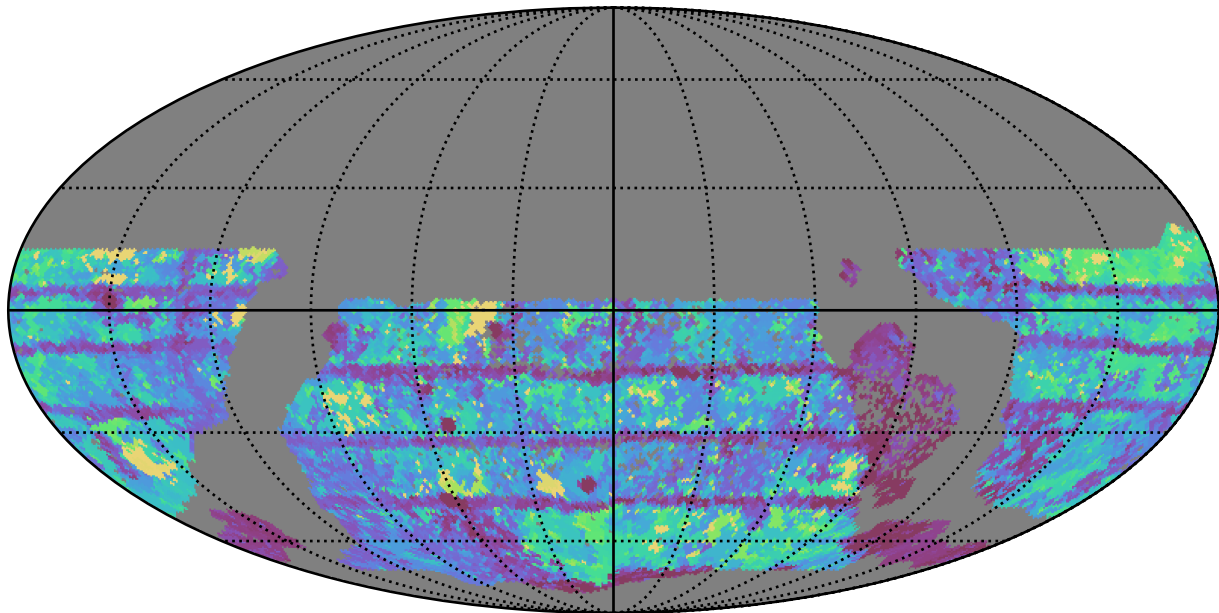
too_combined_s0.5_v3.4_10yrs WFD r band: Max Inter-Night Gap
