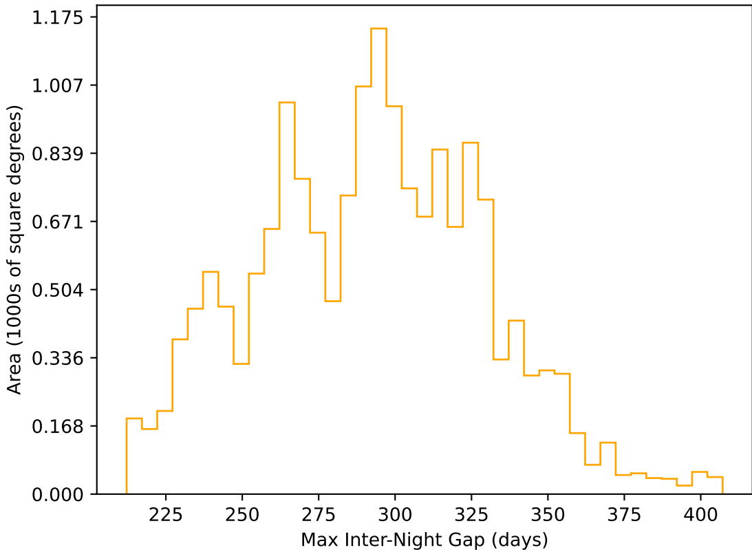
too_combined_s0.5_v3.4_10yrs WFD r band: Max Inter-Night Gap
