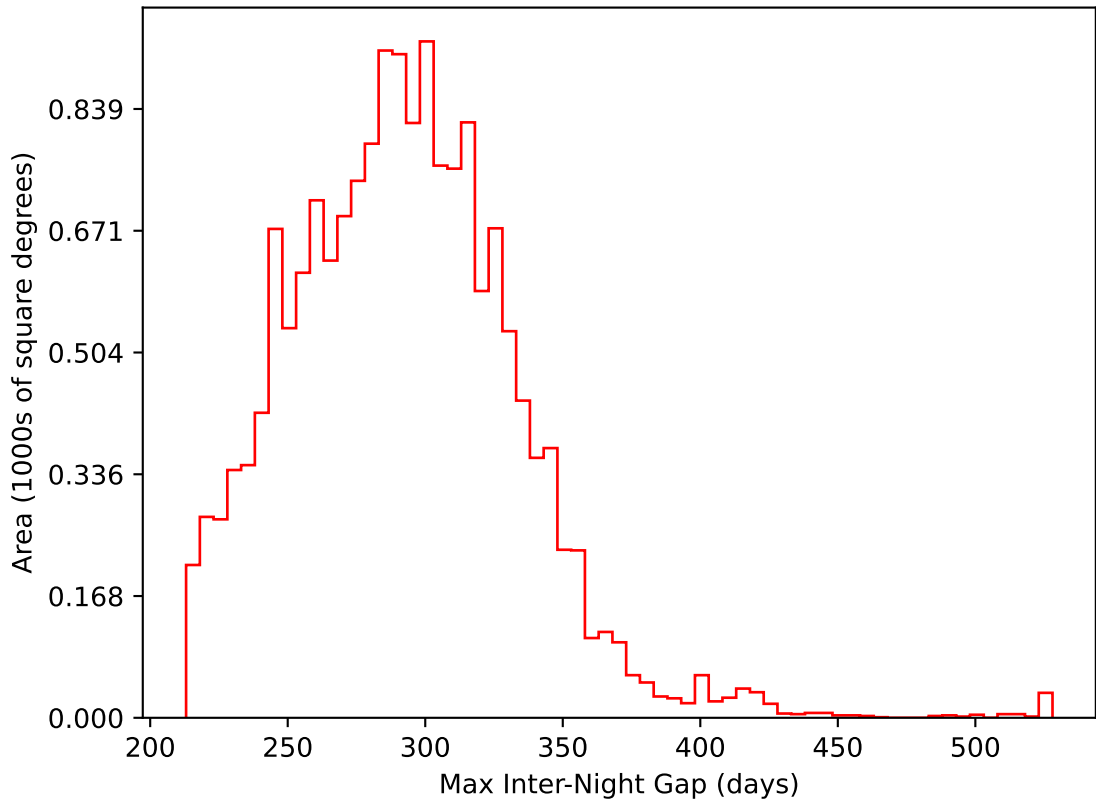
too_combined_s0.5_v3.4_10yrs WFD i band: Max Inter-Night Gap
