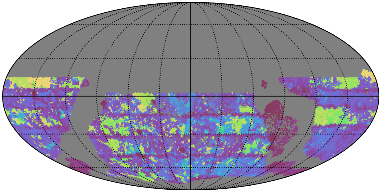
too_combined_s0.5_v3.4_10yrs WFD g band: Max Inter-Night Gap
