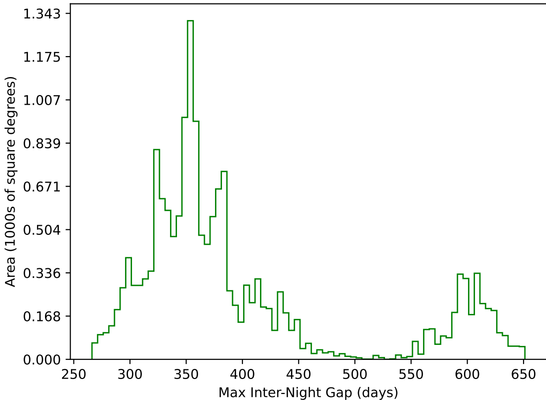
too_combined_s0.5_v3.4_10yrs WFD g band: Max Inter-Night Gap
