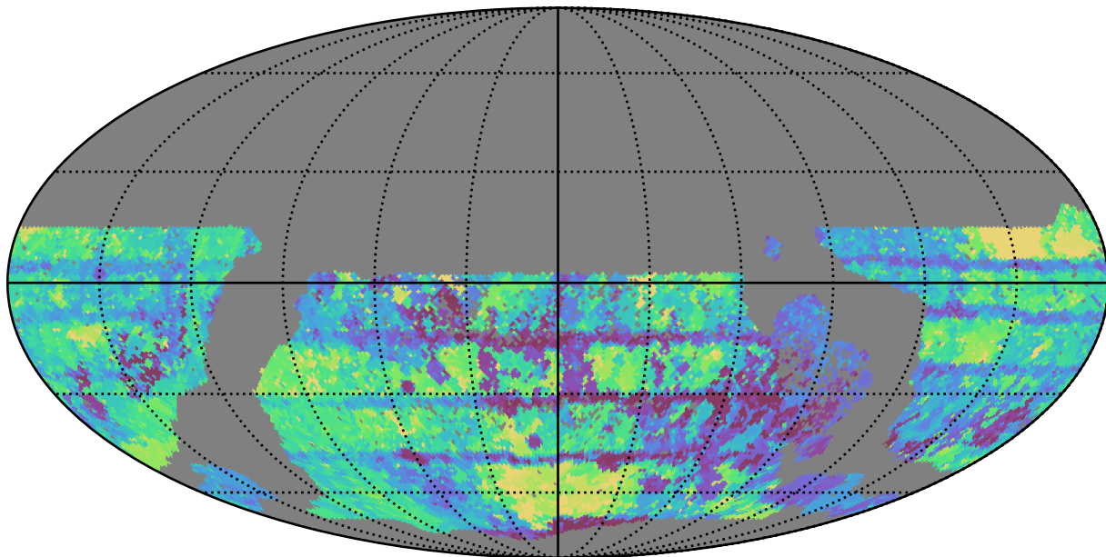
too_combined_s0.5_v3.4_10yrs WFD all bands: Max Inter-Night Gap
