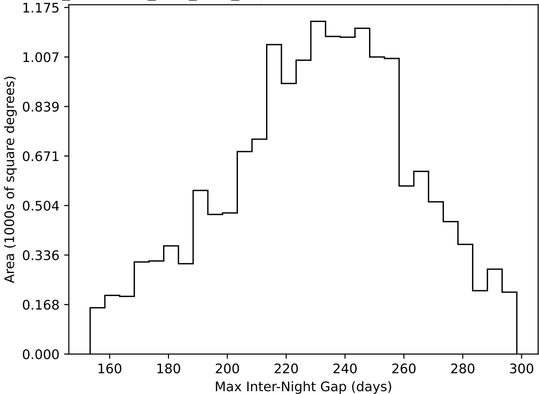
too_combined_s0.5_v3.4_10yrs WFD all bands: Max Inter-Night Gap
