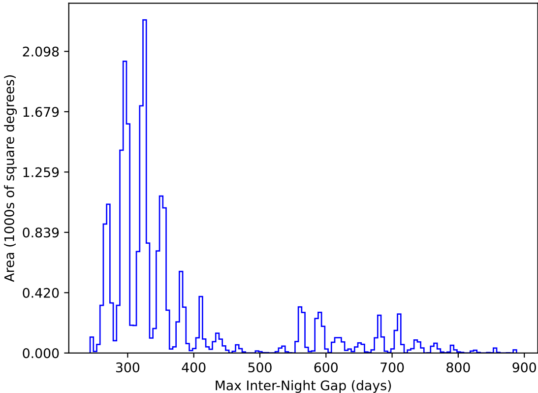
too_combined_s0.5_v3.4_10yrs All sky y band: Max Inter-Night Gap
