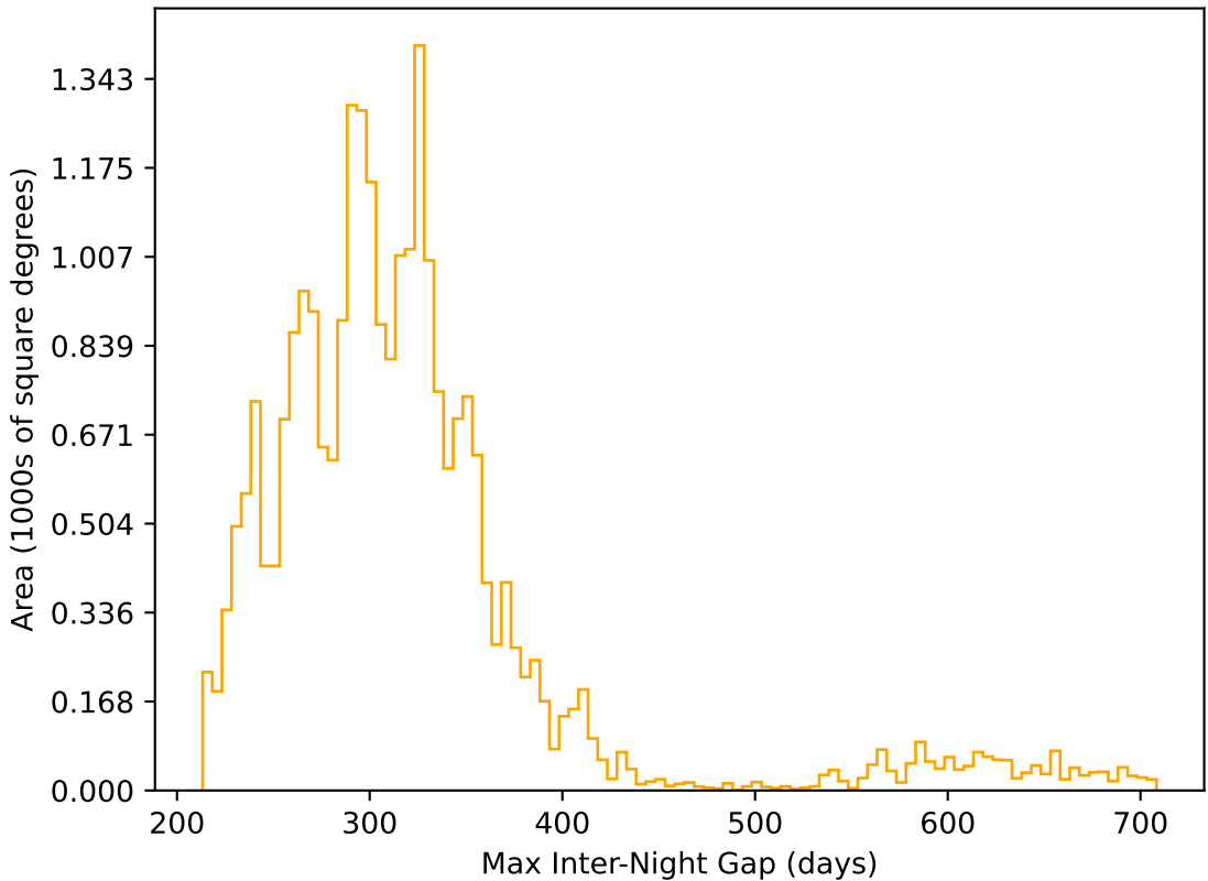
too_combined_s0.5_v3.4_10yrs All sky r band: Max Inter-Night Gap
