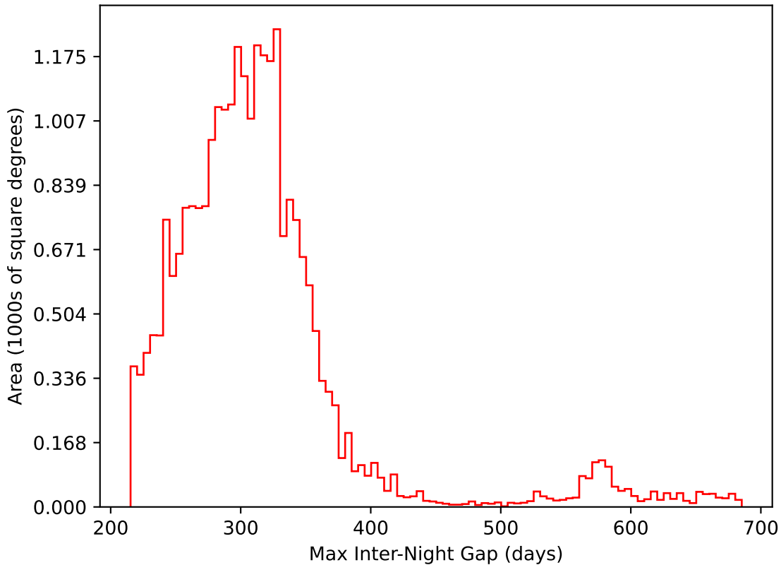
too_combined_s0.5_v3.4_10yrs All sky i band: Max Inter-Night Gap
