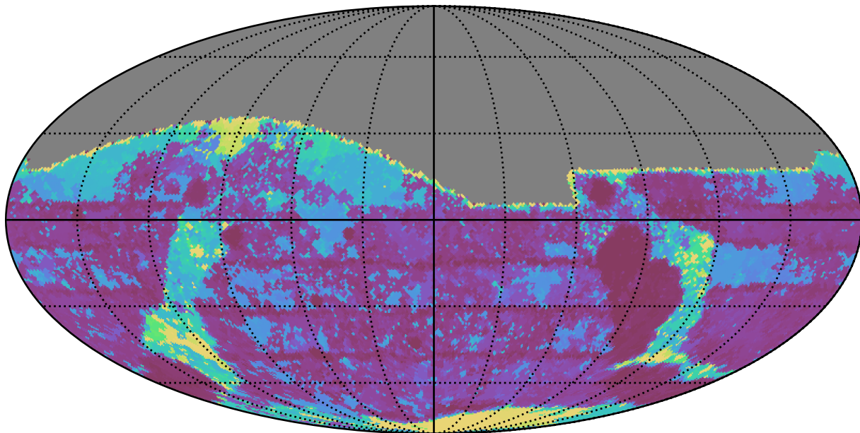
too_combined_s0.5_v3.4_10yrs All sky g band: Max Inter-Night Gap
