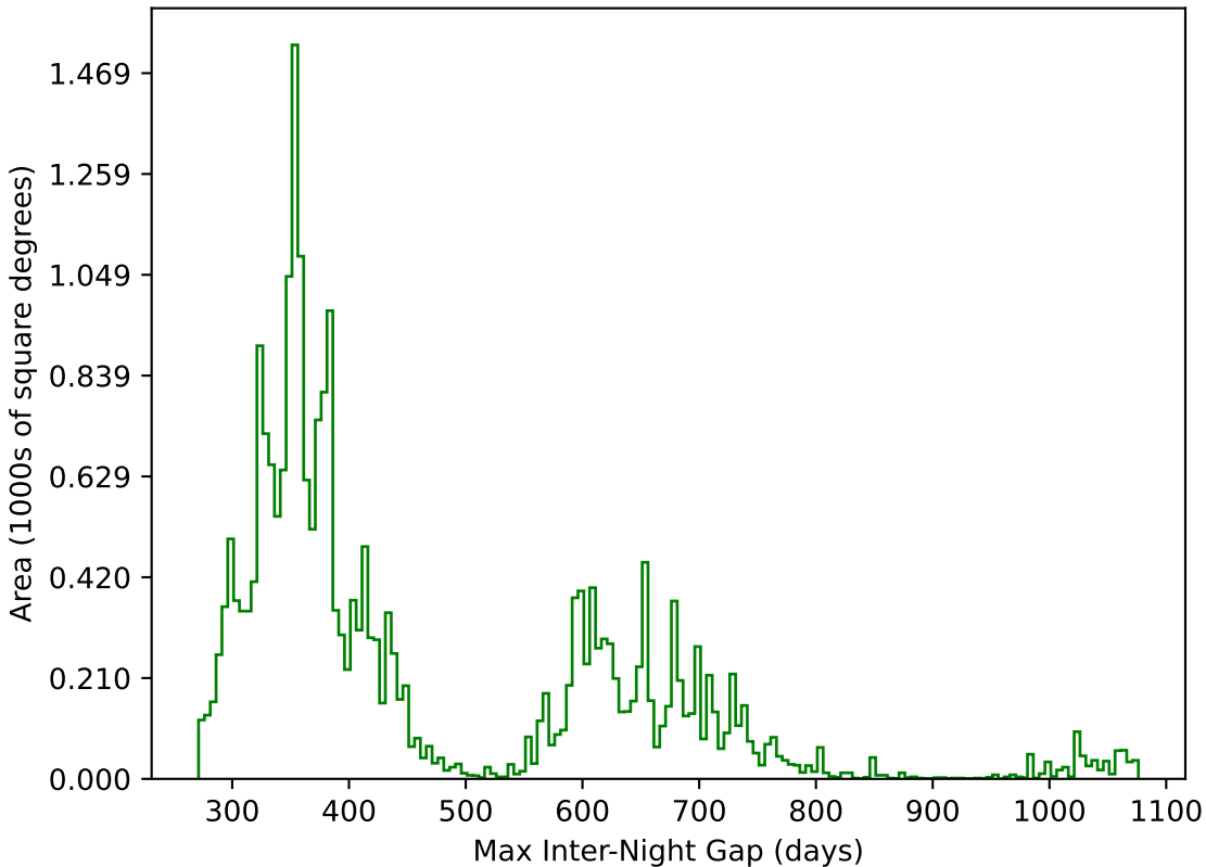
too_combined_s0.5_v3.4_10yrs All sky g band: Max Inter-Night Gap
