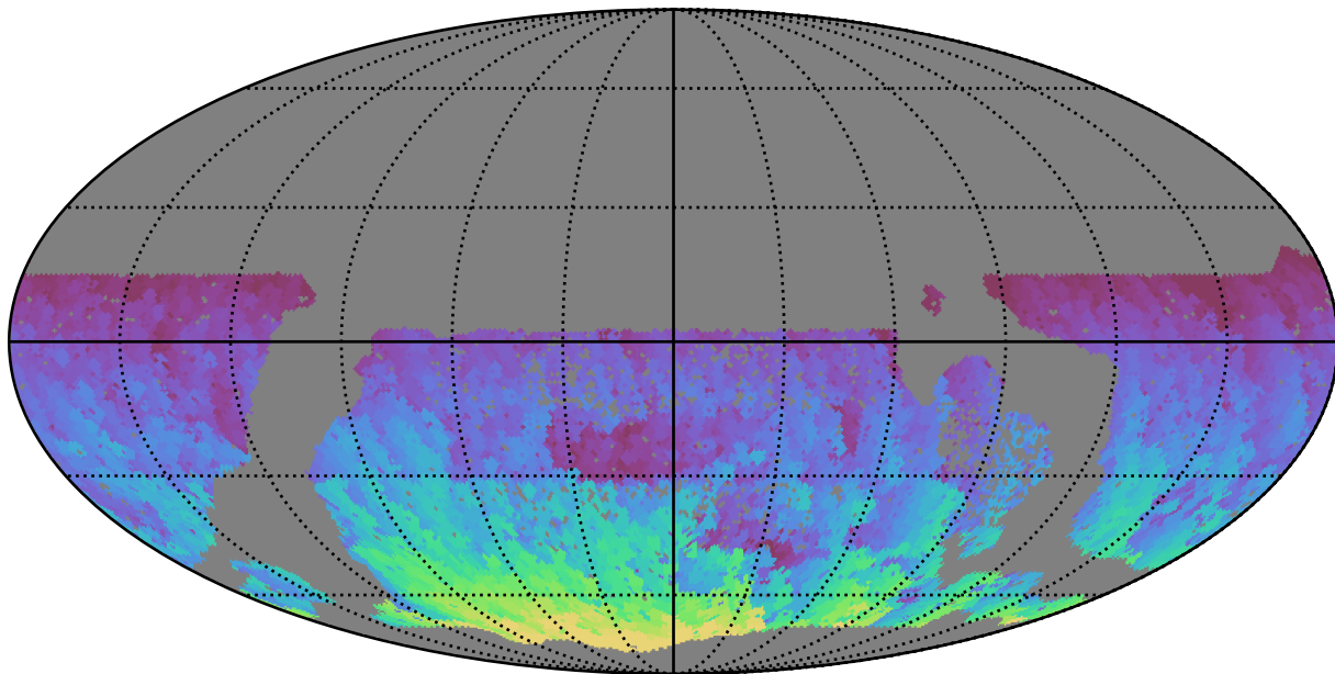
too_combined_s0.5_v3.4_10yrs WFD y band: Max HA
