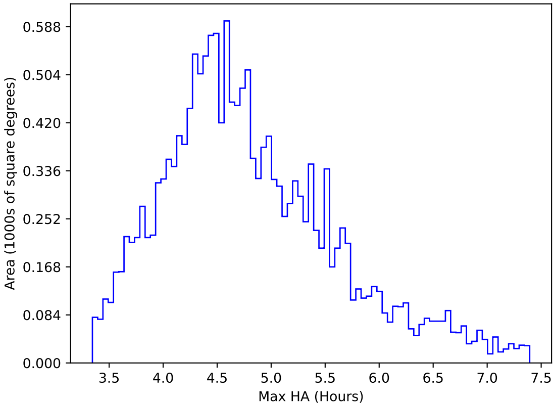
too_combined_s0.5_v3.4_10yrs WFD y band: Max HA
