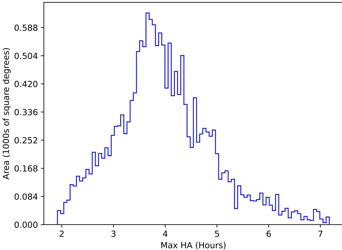
too_combined_s0.5_v3.4_10yrs WFD u band: Max HA
