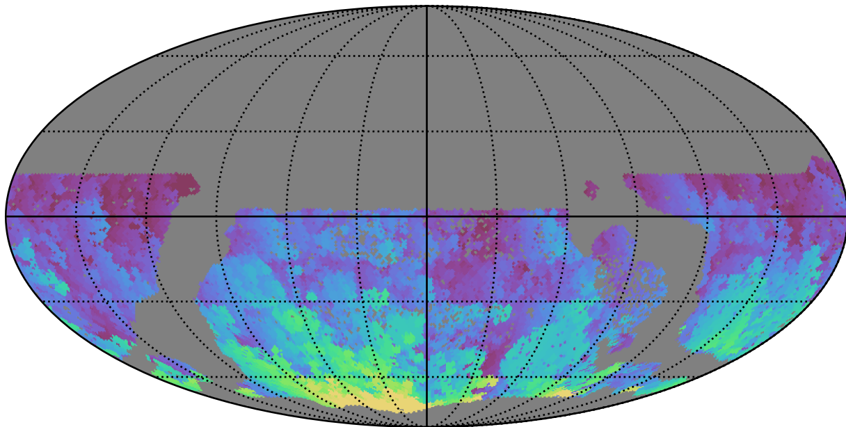
too_combined_s0.5_v3.4_10yrs WFD g band: Max HA
