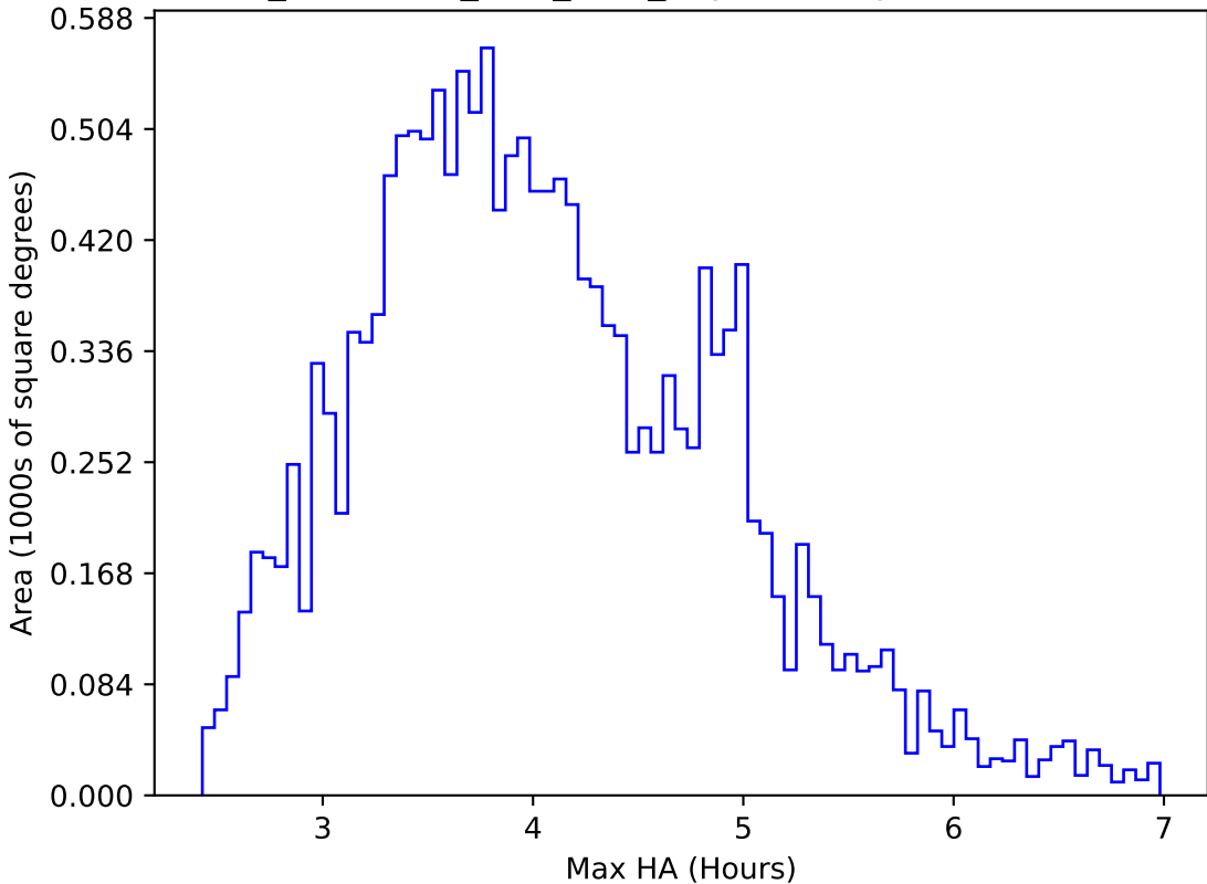
too_combined_s0.5_v3.4_10yrs WFD g band: Max HA
