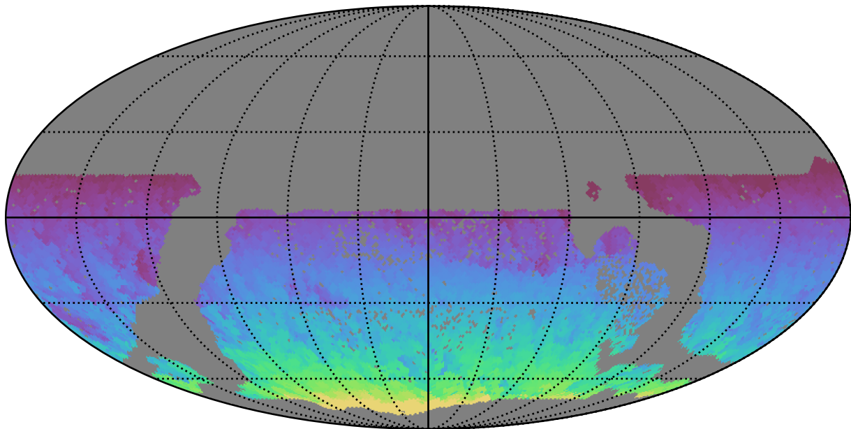
too_combined_s0.5_v3.4_10yrs WFD all bands: Max HA
