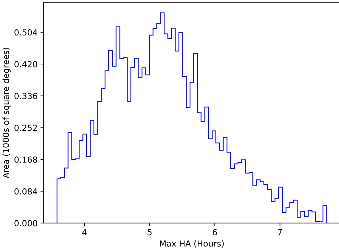
too_combined_s0.5_v3.4_10yrs WFD all bands: Max HA
