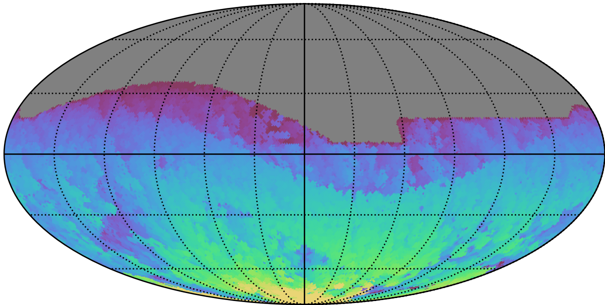
too_combined_s0.5_v3.4_10yrs All sky z band: Max HA
