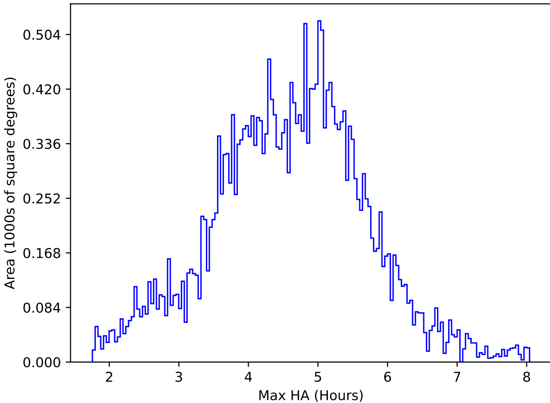
too_combined_s0.5_v3.4_10yrs All sky z band: Max HA
