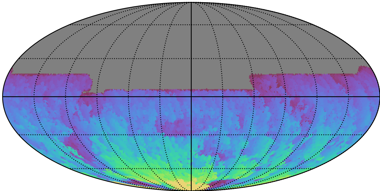
too_combined_s0.5_v3.4_10yrs All sky y band: Max HA
