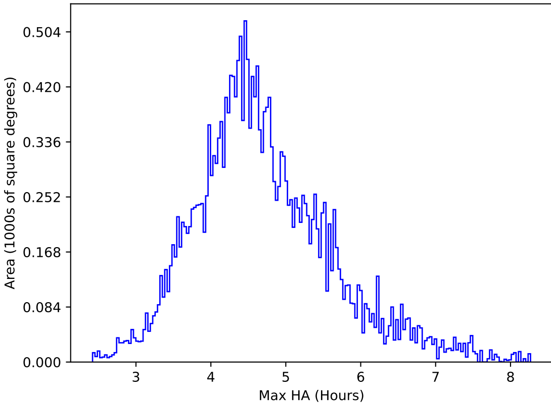
too_combined_s0.5_v3.4_10yrs All sky y band: Max HA
