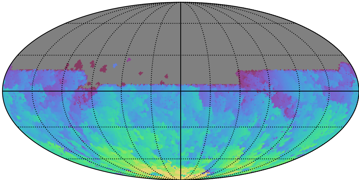
too_combined_s0.5_v3.4_10yrs All sky u band: Max HA
