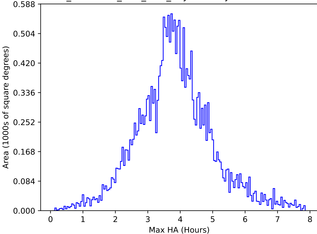
too_combined_s0.5_v3.4_10yrs All sky u band: Max HA
