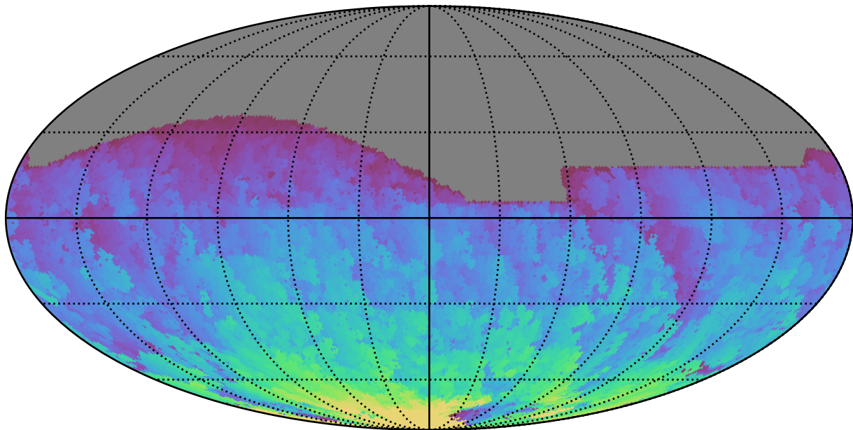
too_combined_s0.5_v3.4_10yrs All sky r band: Max HA
