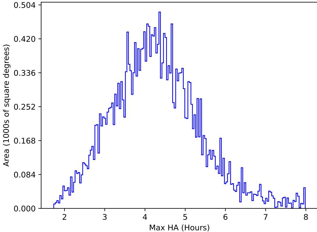
too_combined_s0.5_v3.4_10yrs All sky r band: Max HA
