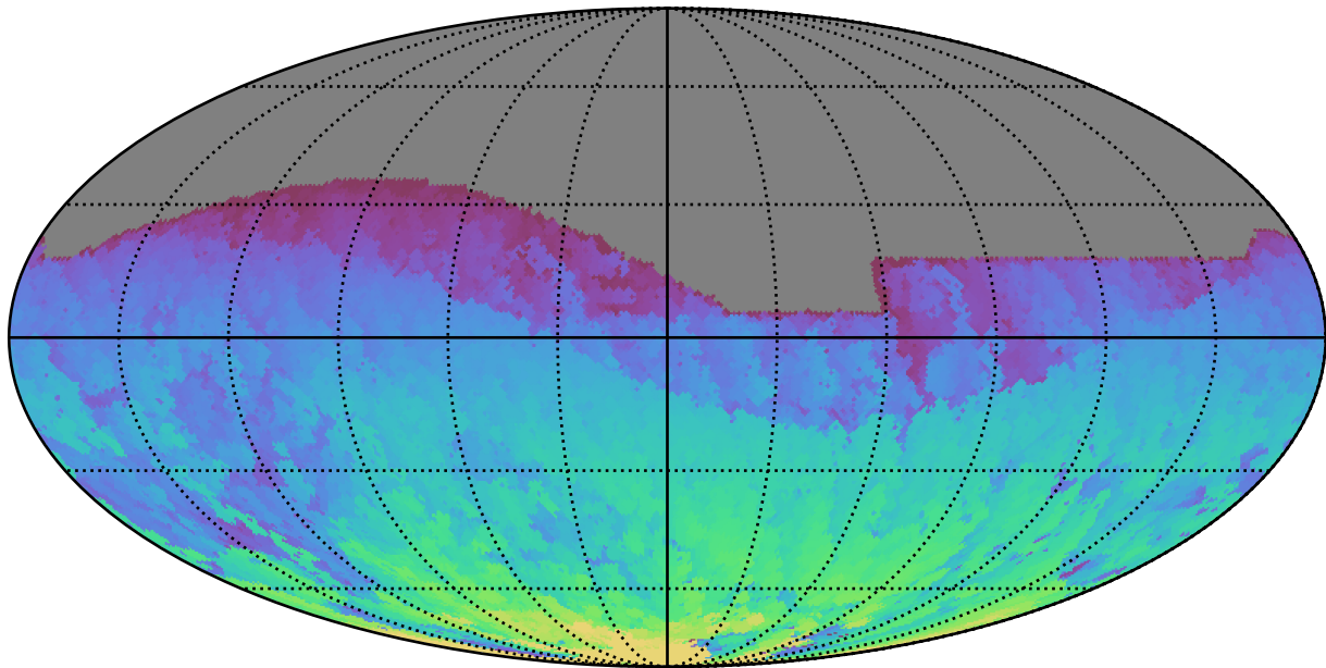
too_combined_s0.5_v3.4_10yrs All sky i band: Max HA
