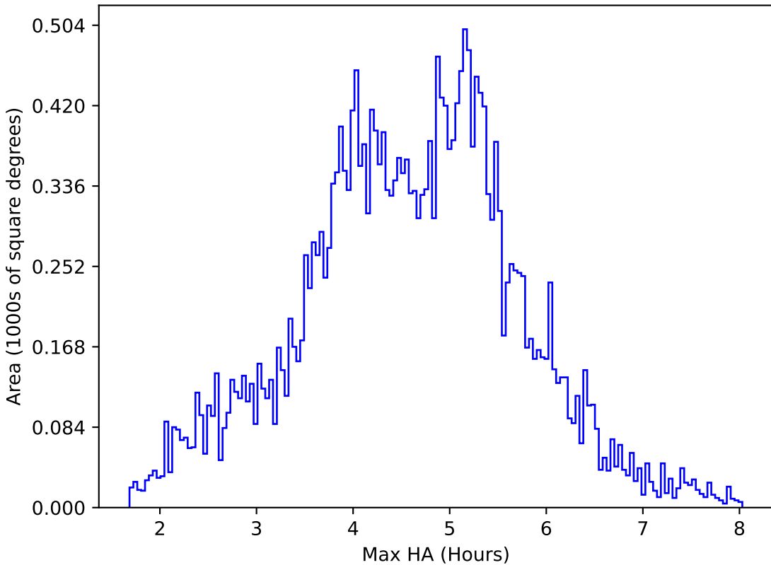
too_combined_s0.5_v3.4_10yrs All sky i band: Max HA
