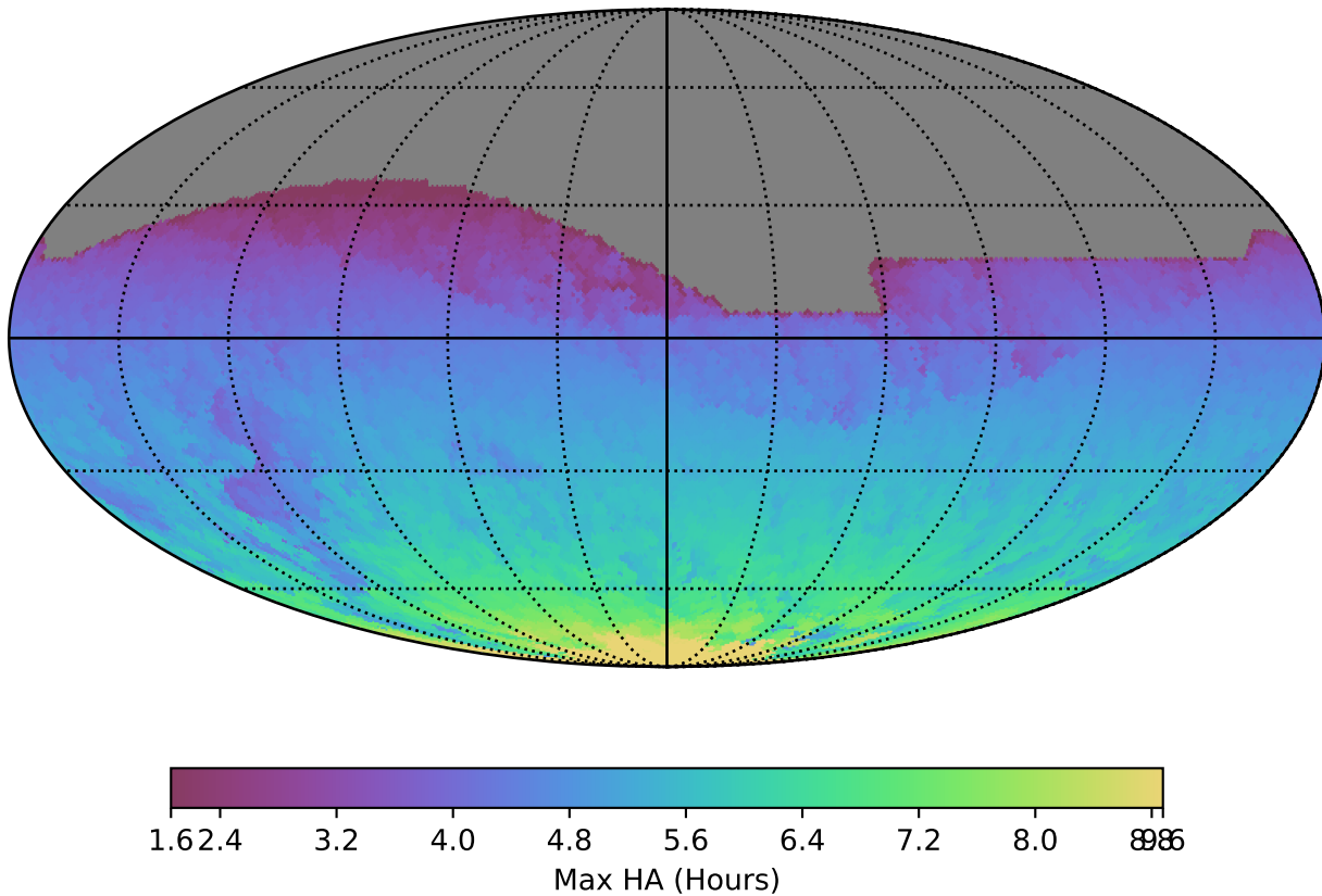
too_combined_s0.5_v3.4_10yrs All sky all bands: Max HA
