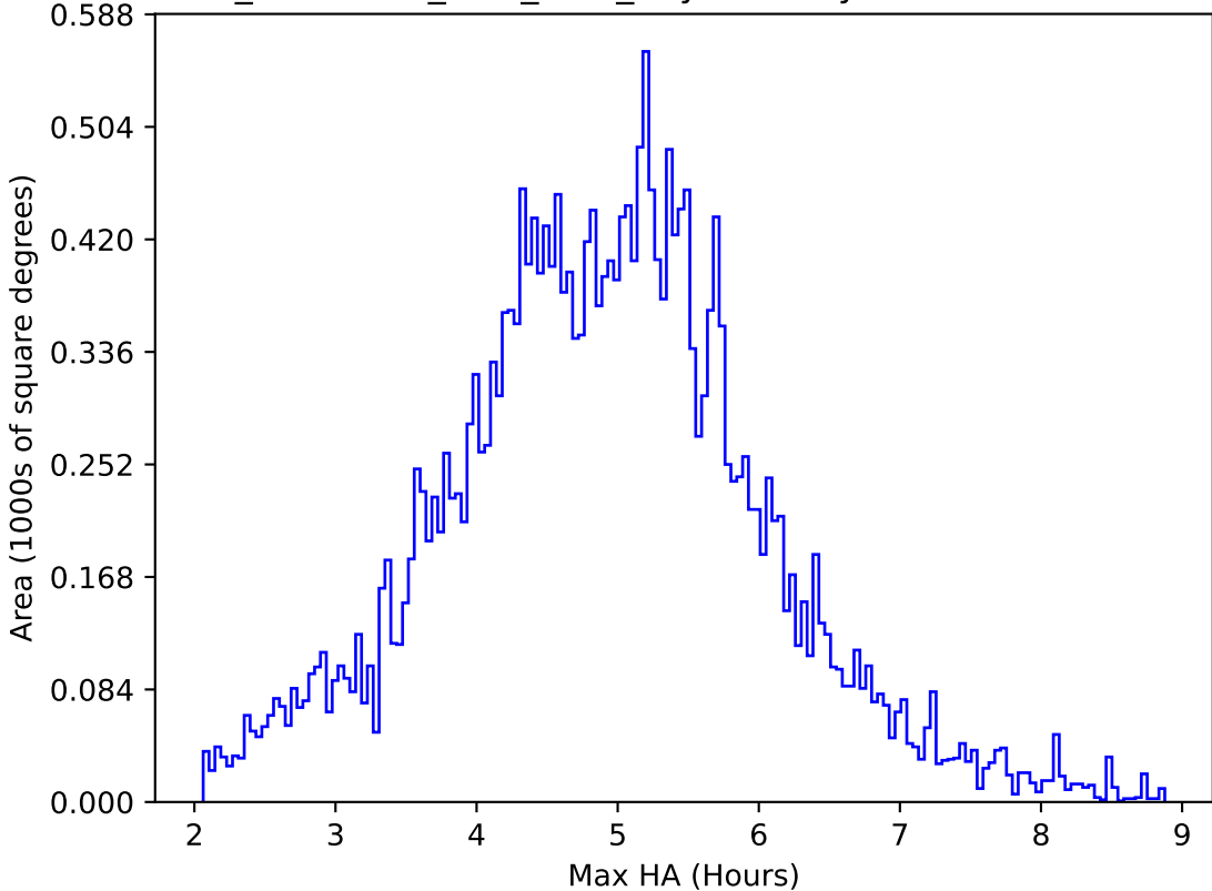
too_combined_s0.5_v3.4_10yrs All sky all bands: Max HA
