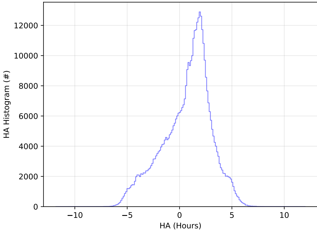
too_combined_s0.5_v3.4_10yrs WFD z band: HA Histogram
