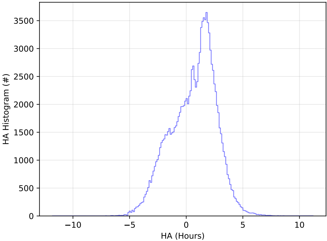
too_combined_s0.5_v3.4_10yrs WFD u band: HA Histogram
