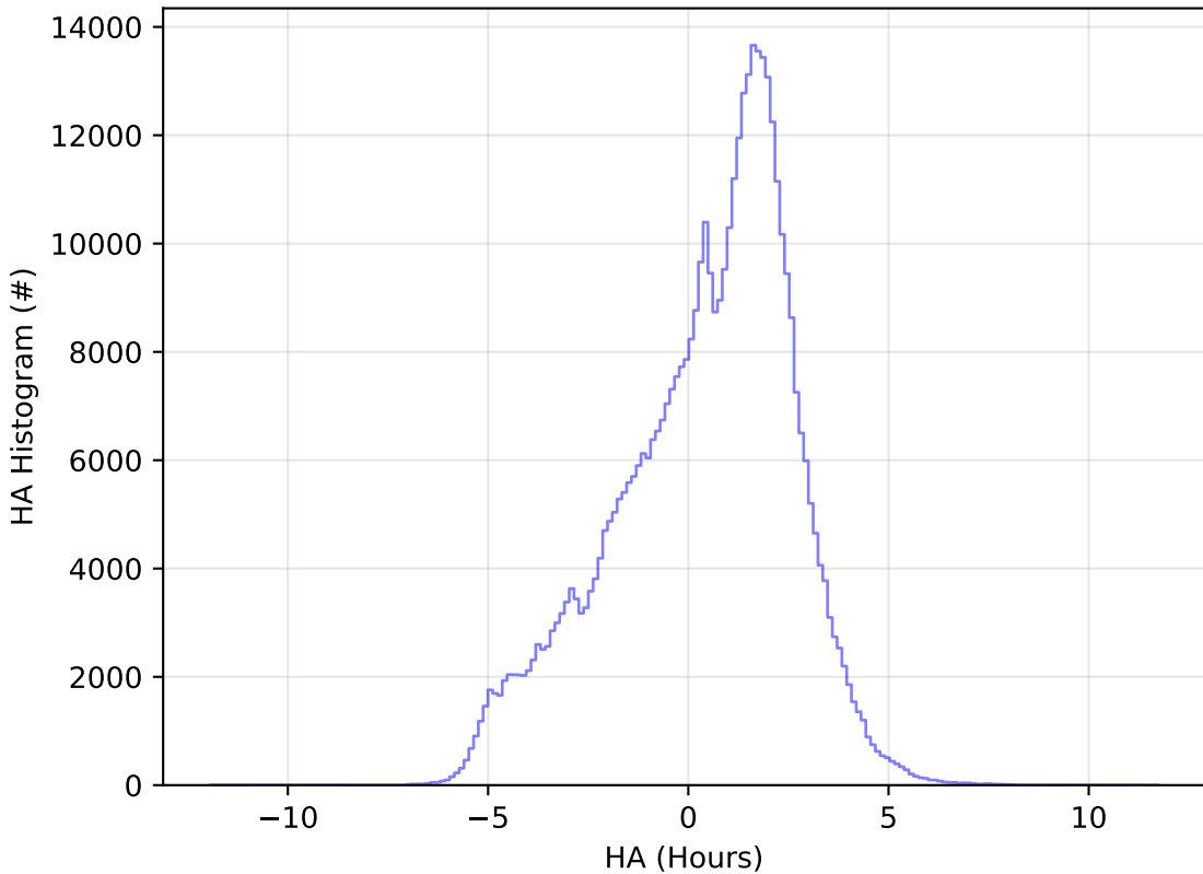
too_combined_s0.5_v3.4_10yrs WFD r band: HA Histogram
