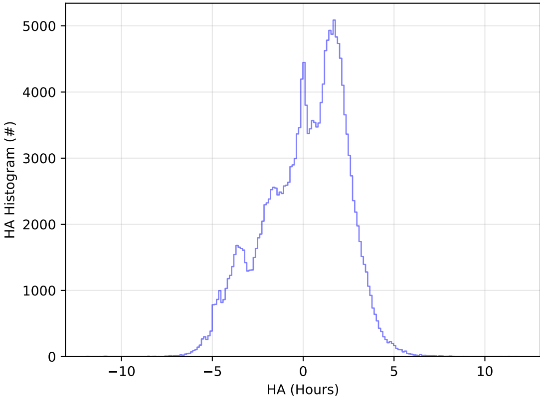
too_combined_s0.5_v3.4_10yrs WFD g band: HA Histogram
