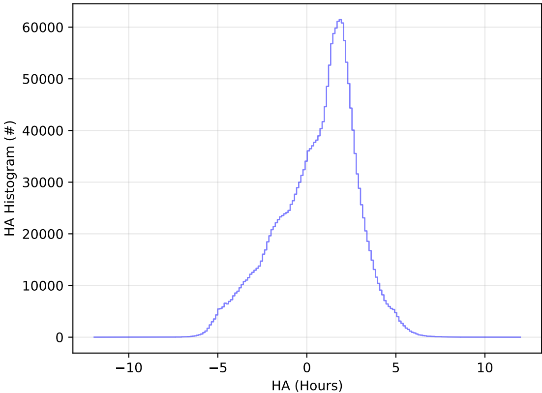
too_combined_s0.5_v3.4_10yrs WFD all bands: HA Histogram
